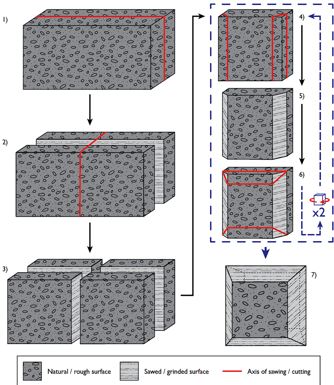
Figure 5. Visualization for protocol used to create standardized basalt blanks (which would also apply to other types of stones).
