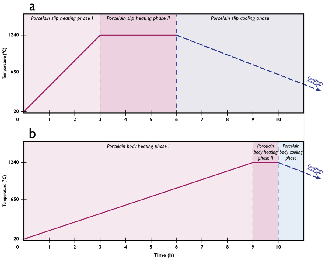
Figure 11. Heating curves for the firing of porcelain blanks, including the curve used for (a) white porcelain slip and (b) black porcelain body.
