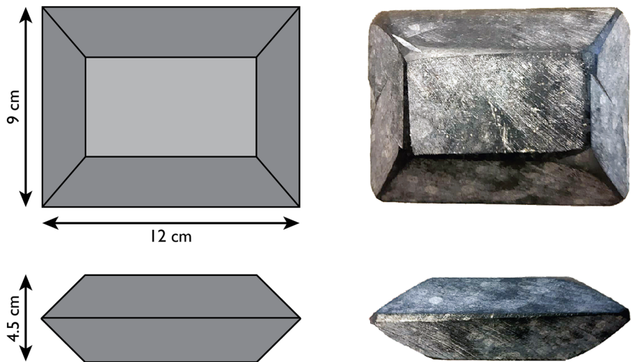
Figure 4. Schematized and actual polyhedral basalt blank made using a diamond saw and grinder.
