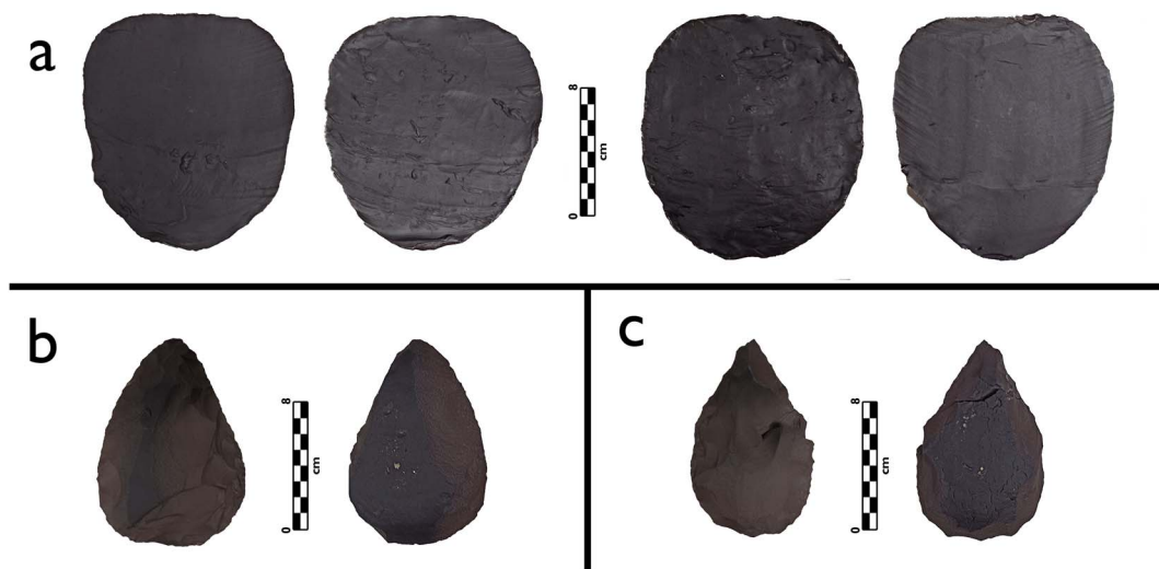
Figure 13. (a) Four fired black porcelain blanks in the form of large flakes with the (b, c) ventral and dorsal view of two said blanks knapped into simple bifaces..
